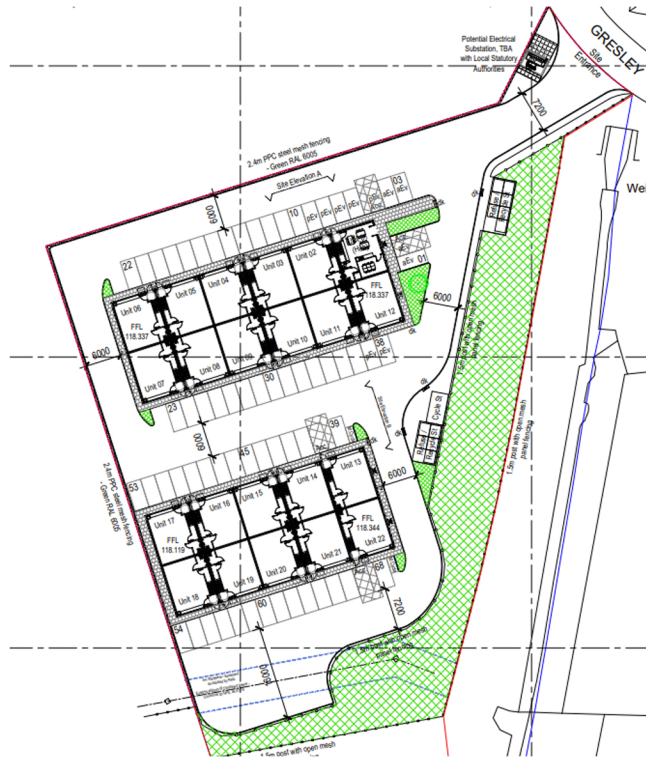
SITE LAYOUT
